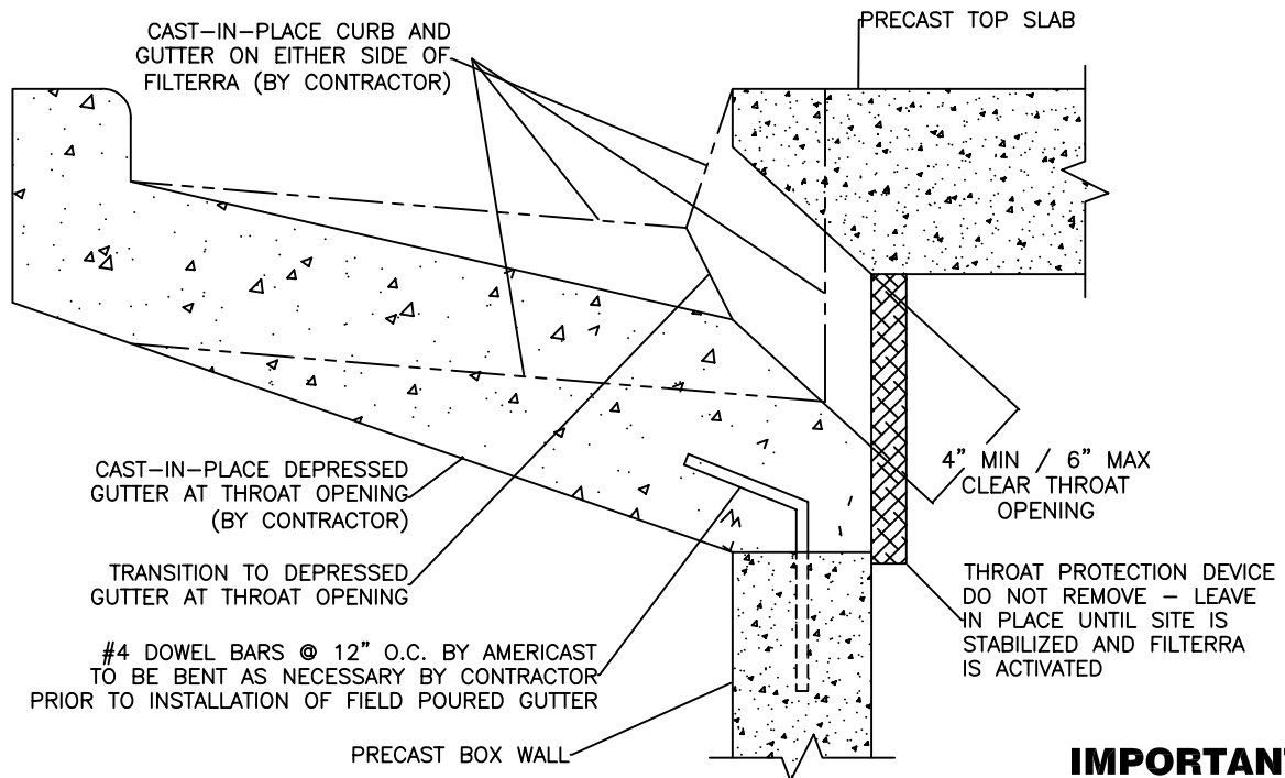
FLUME SECTION VIEW FILTERRA THROAT OPENING
